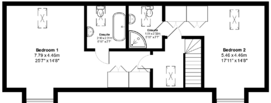
FIRST FLOOR
